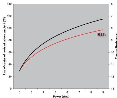
HeatSink Performance
